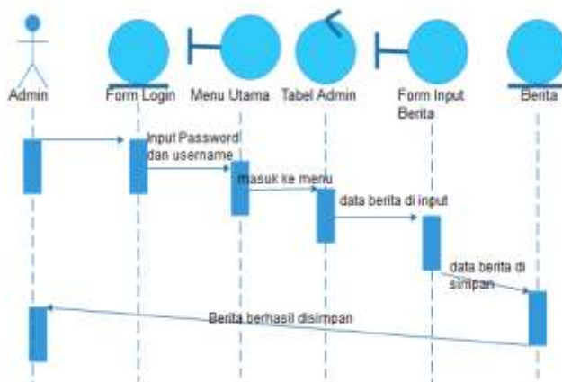
Gbr. 4 Merancang Sequence Diagram
