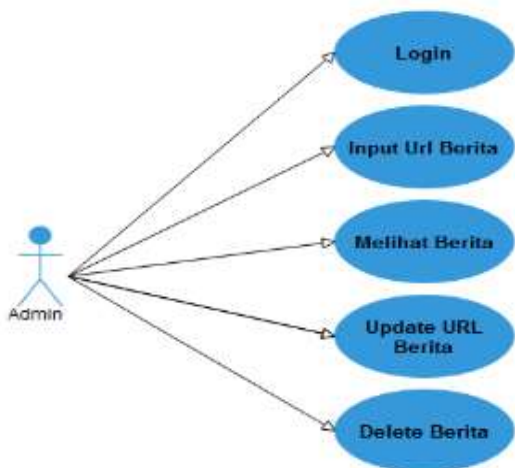
Gbr. 2 Merancang Use Case Diagram
