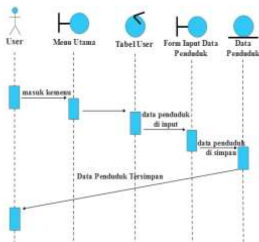
Gambar 5. Sequence Diagram
