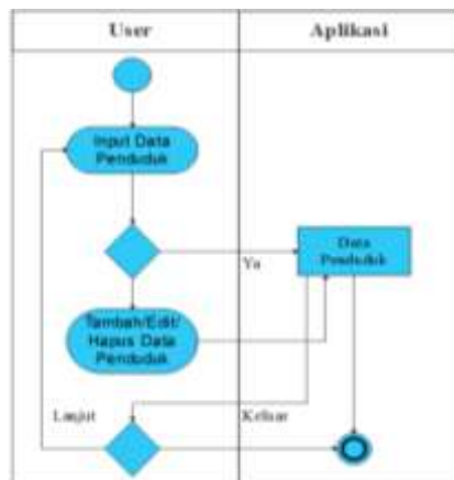
Gambar 3. Activity Diagram
