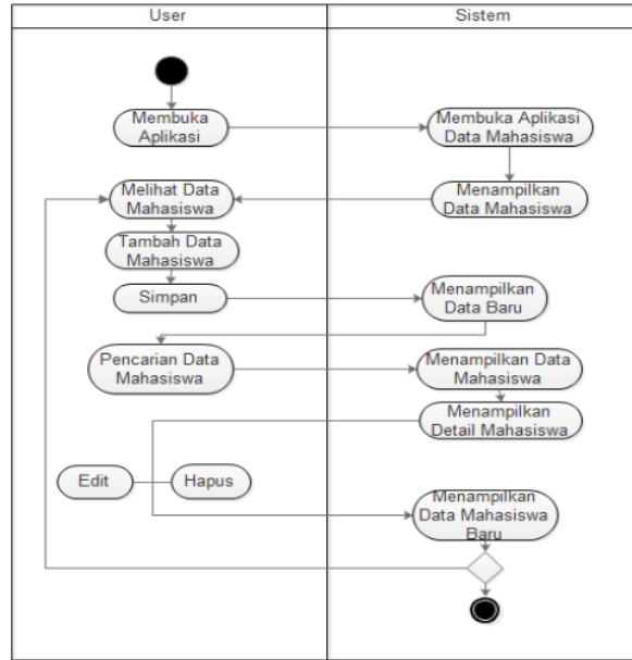
Gambar 3. Activity Diagram
