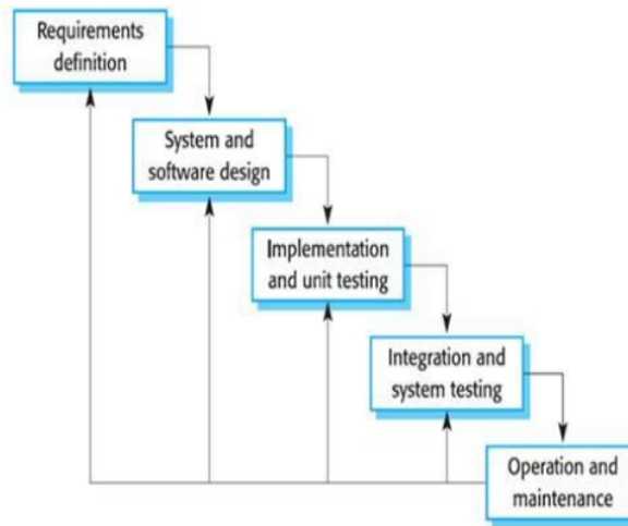
Gambar 1. Metode Waterfall
