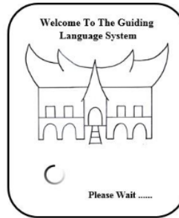
Figure 6. Splash Screen
