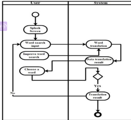
Figure 3. Activity Diagram
