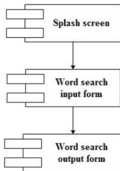
Figure 5. Component Diagram
