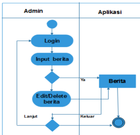
Gbr. 3 Merancang Activity Diagram
