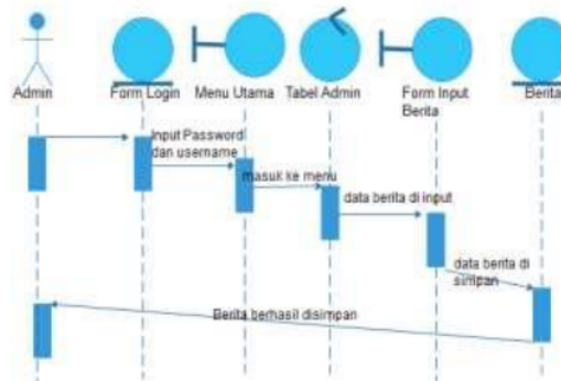
Gbr. 4 Merancang Sequence Diagram
